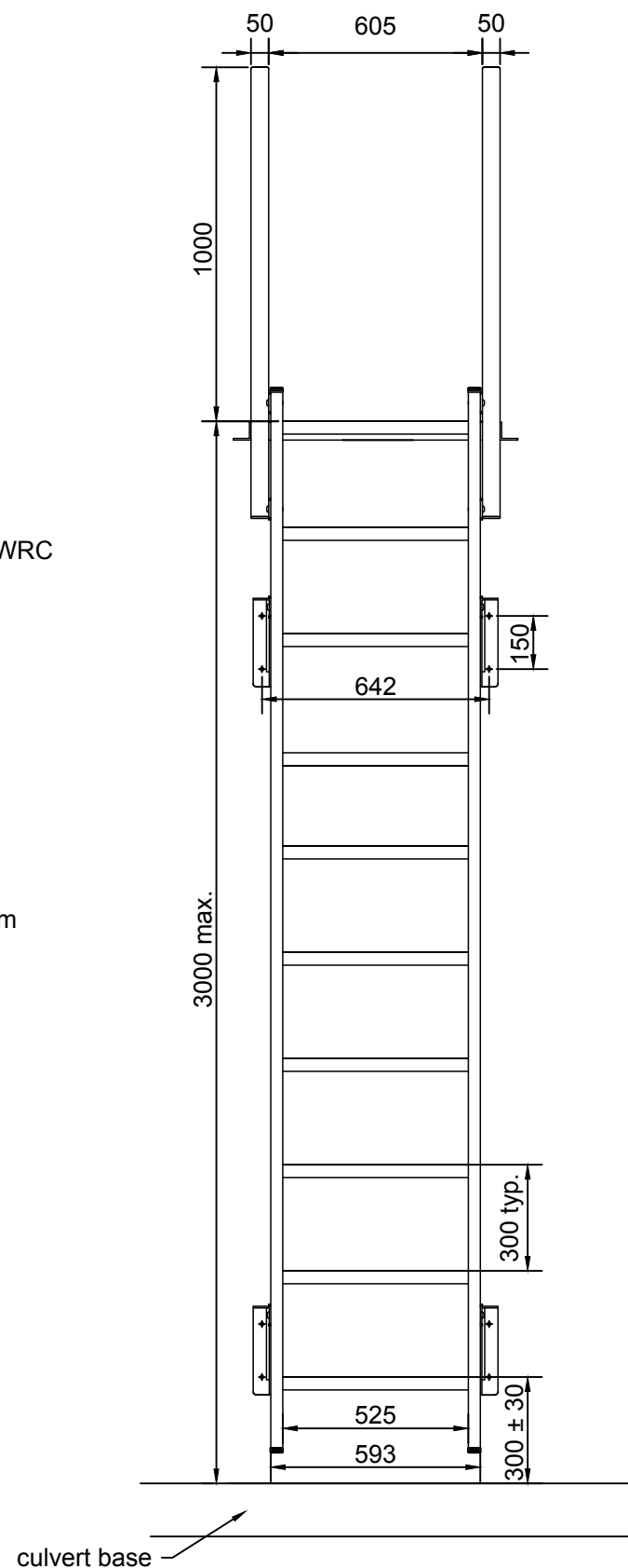
2 Ladder Front view
