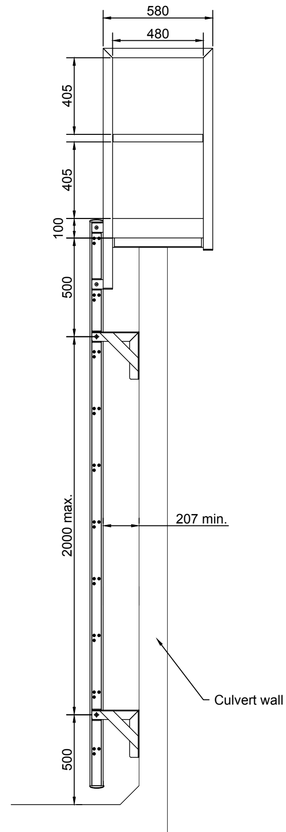
3 Ladder Side View
