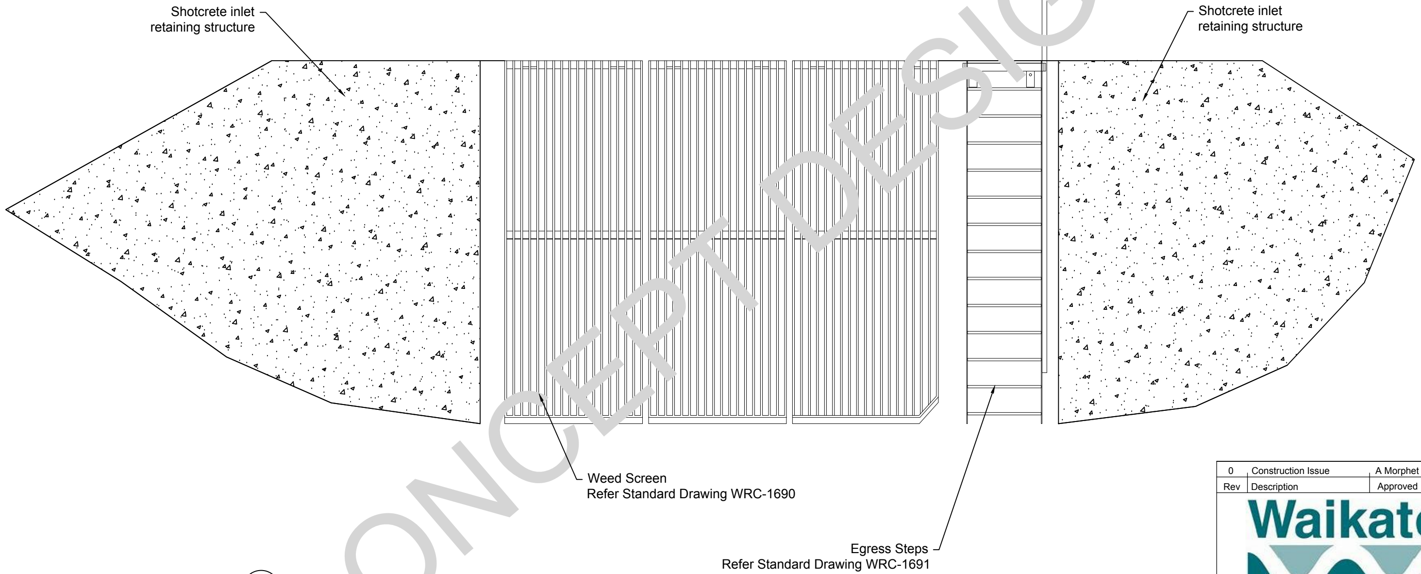
3 Inlet Elevation
