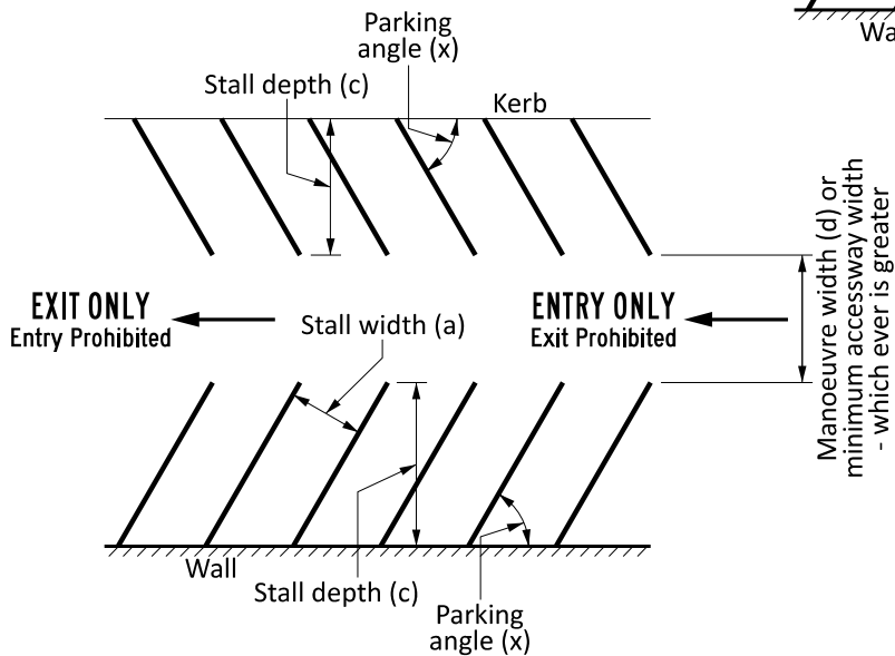
DOUBLE ROW ONE WAY ENTRY
