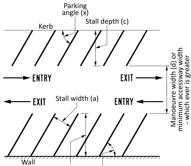
DOUBLE ROW TWO WAY ENTRY
