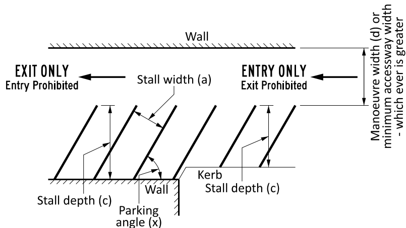
SINGLE ROW ONE WAY ENTRY
