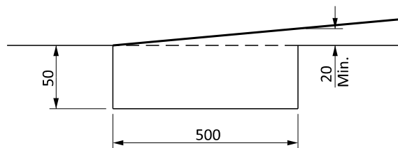
EXISTING PAVEMENT KEY-IN
