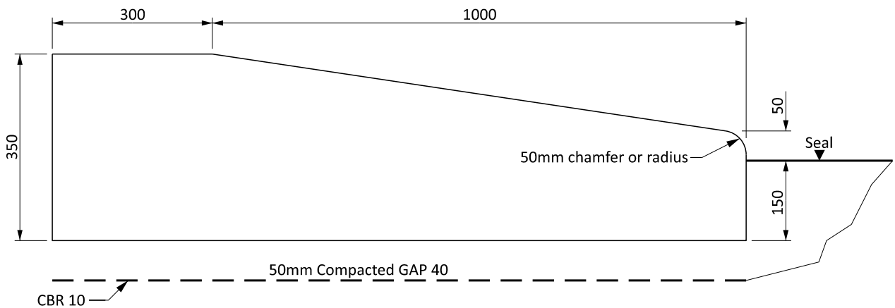
CONCRETE ROTARY COLLAR
