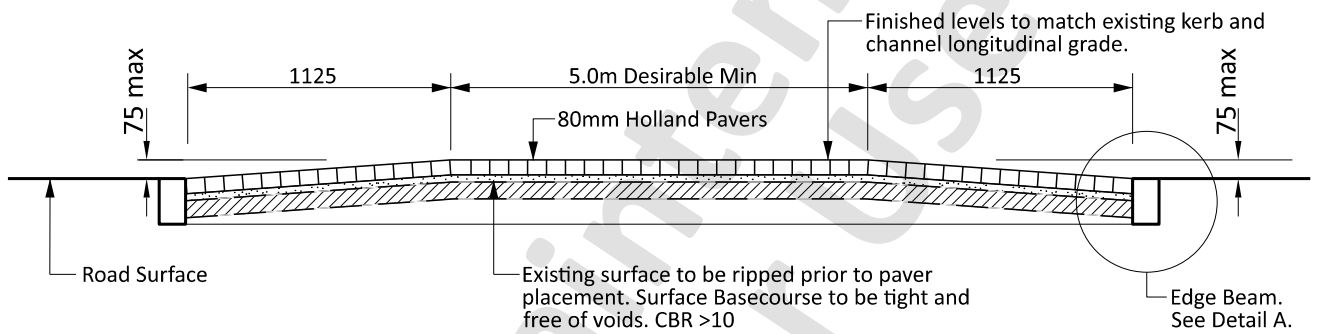
SECTION A - A (RAISED PEDESTRIAN RAMP)
