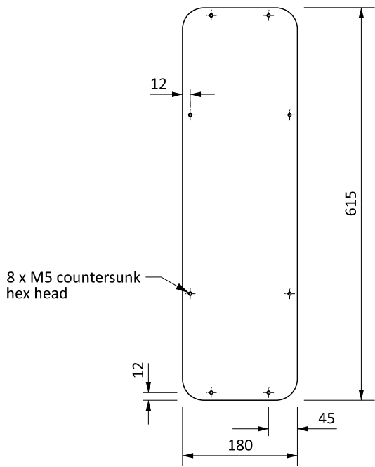
Hatch Cover 5.8mm Plate
