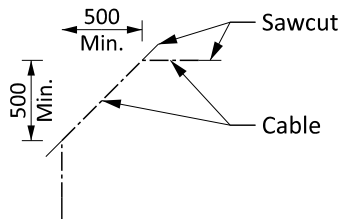
LOOP CORNER DETAIL
