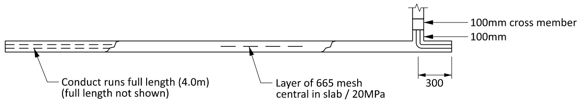
FRONT ELEVATION
