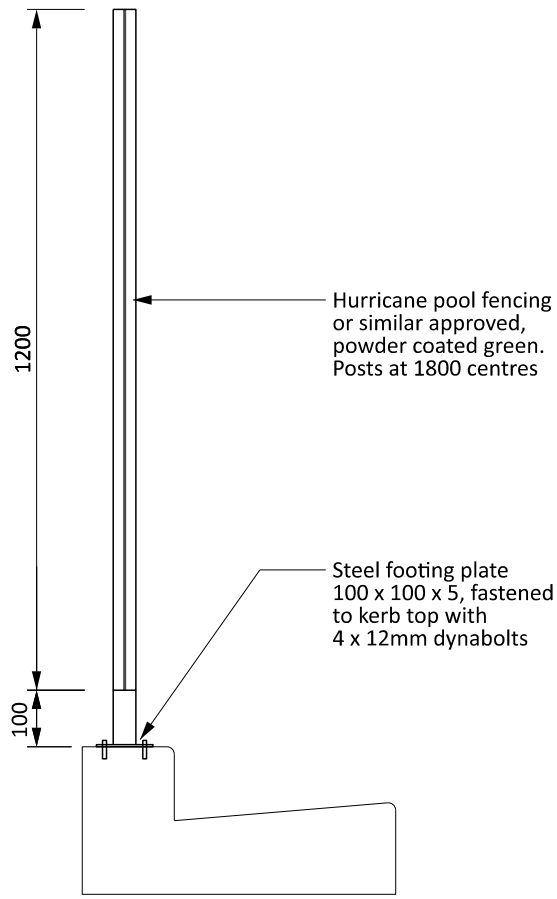
KERB TOP
