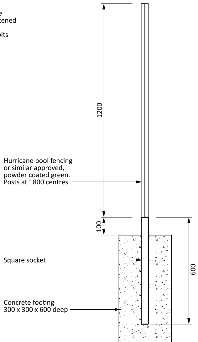
FOOTING MOUNTED
