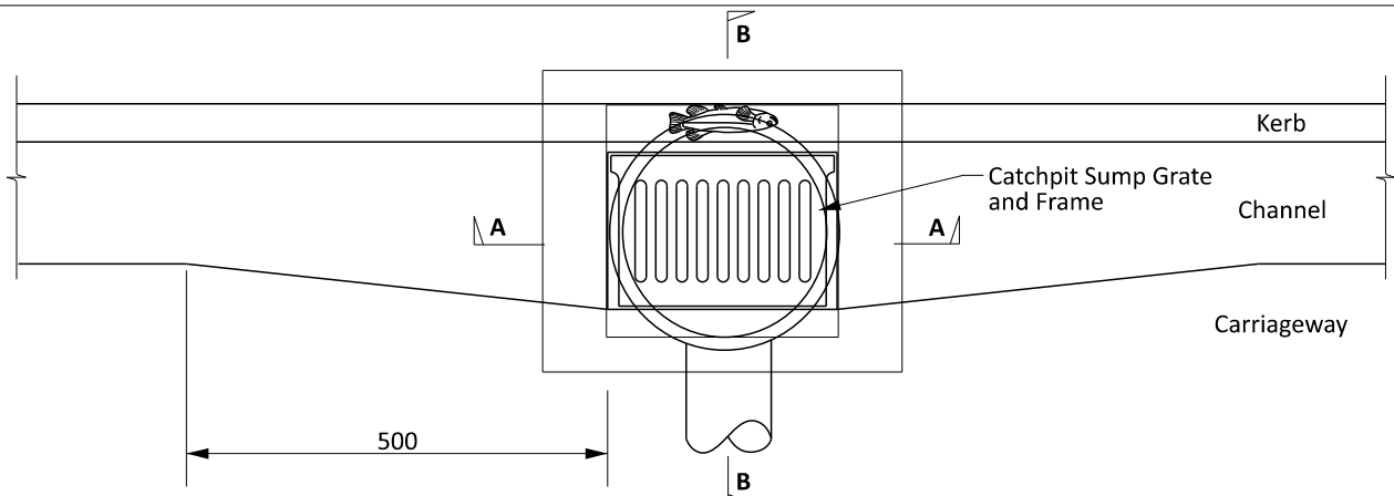
PLAN SCALE 1:25
