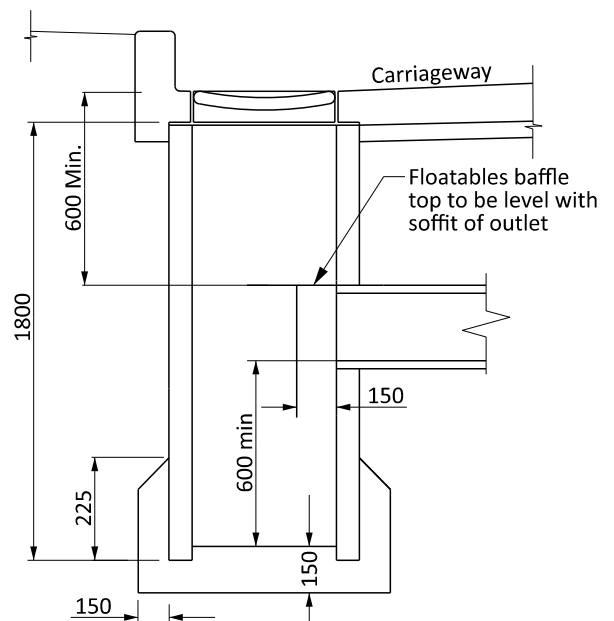
SECTION B-B SCALE 1:25
