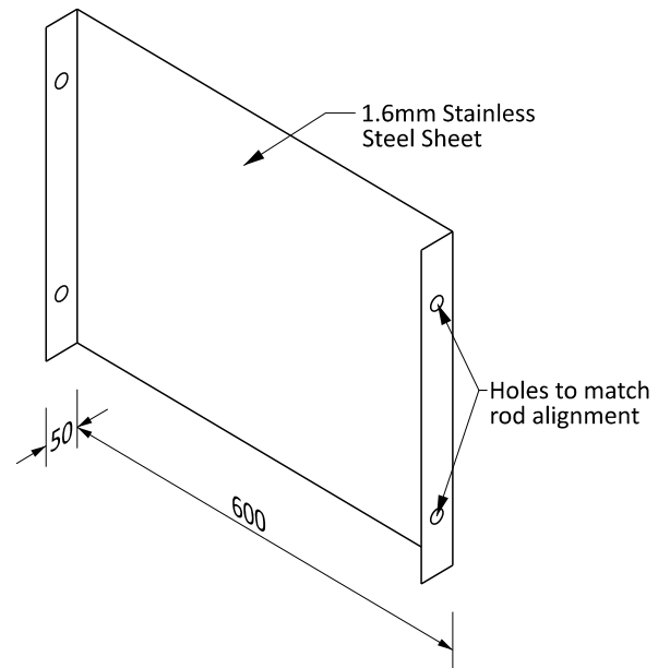
FLOATABLES BAFFLE DETAIL Not to Scale
