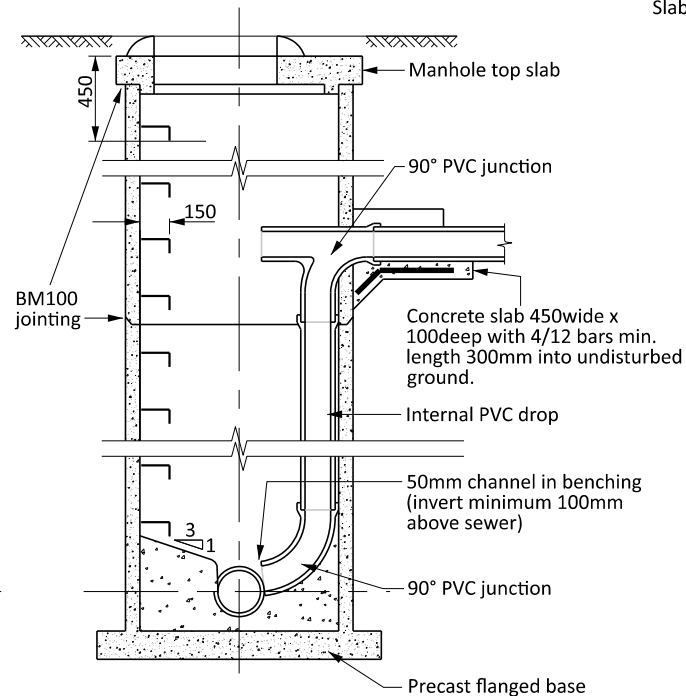
DROP MANHOLES
