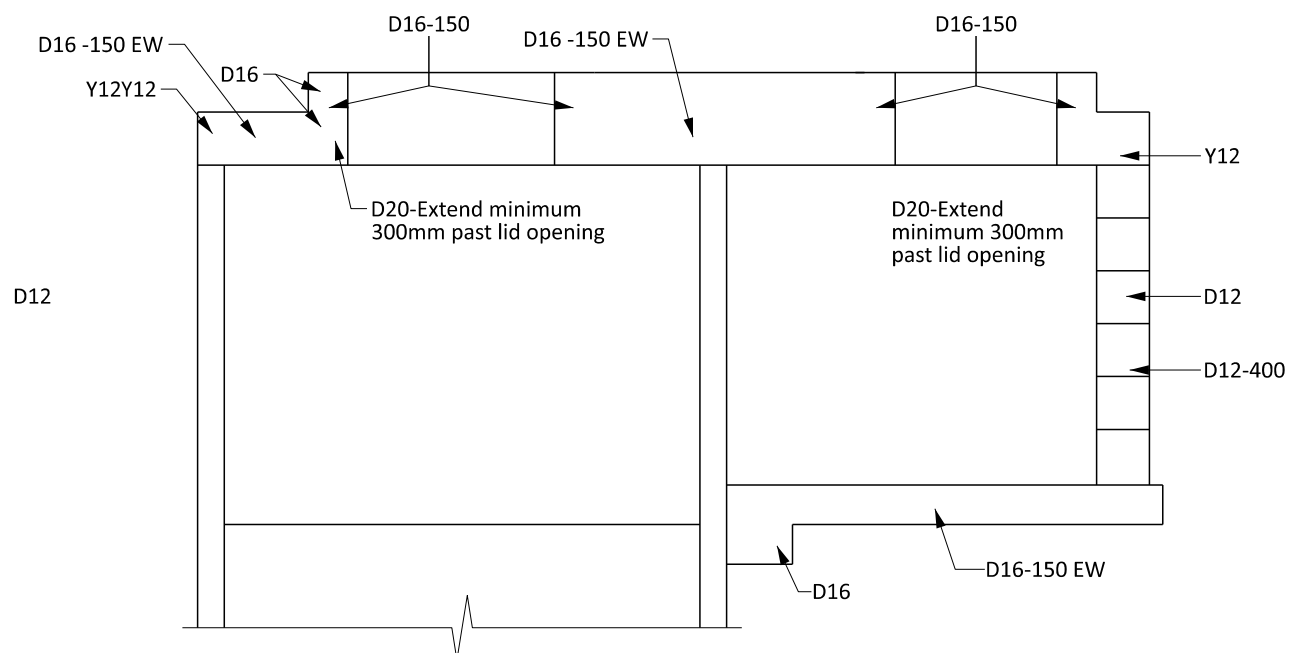
SECTION A
