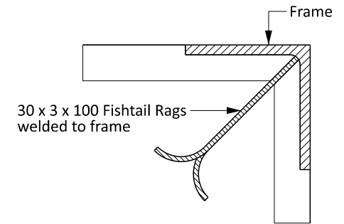
FISHTAIL RAG TYPICAL DETAIL
