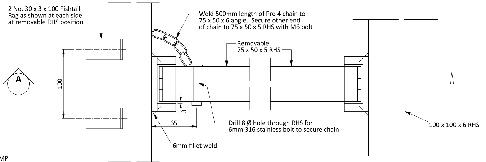
DETAIL 1
