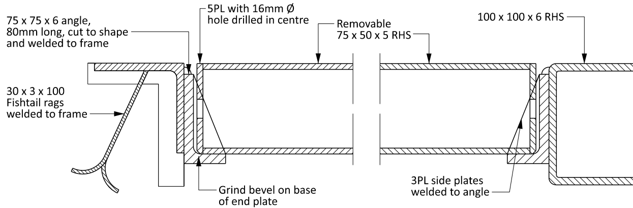
SECTION A
