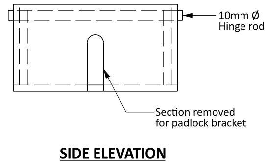
PADLOCK BOX TYPICAL DETAIL
