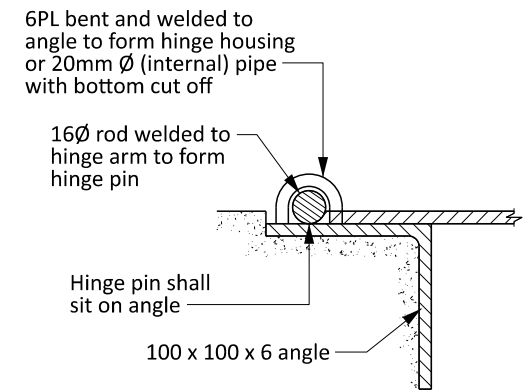
LID HINGE TYPICAL DETAIL
