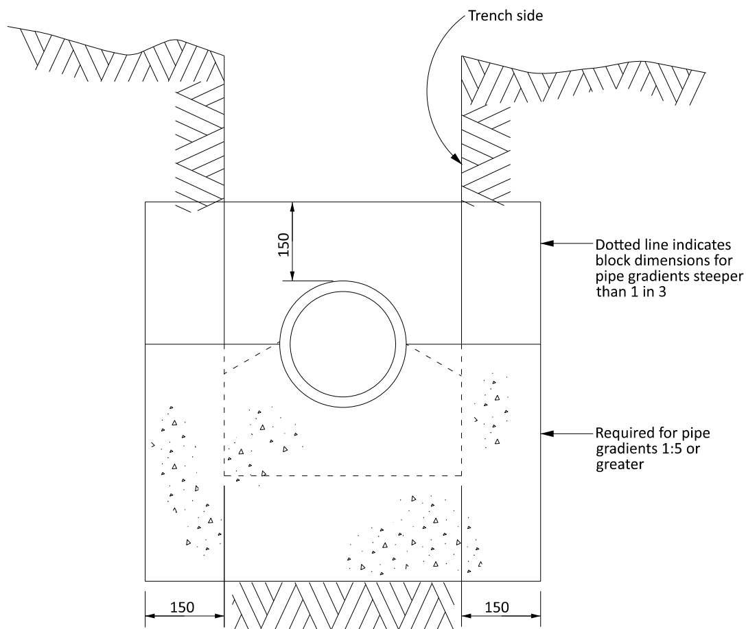
CROSS SECTION
