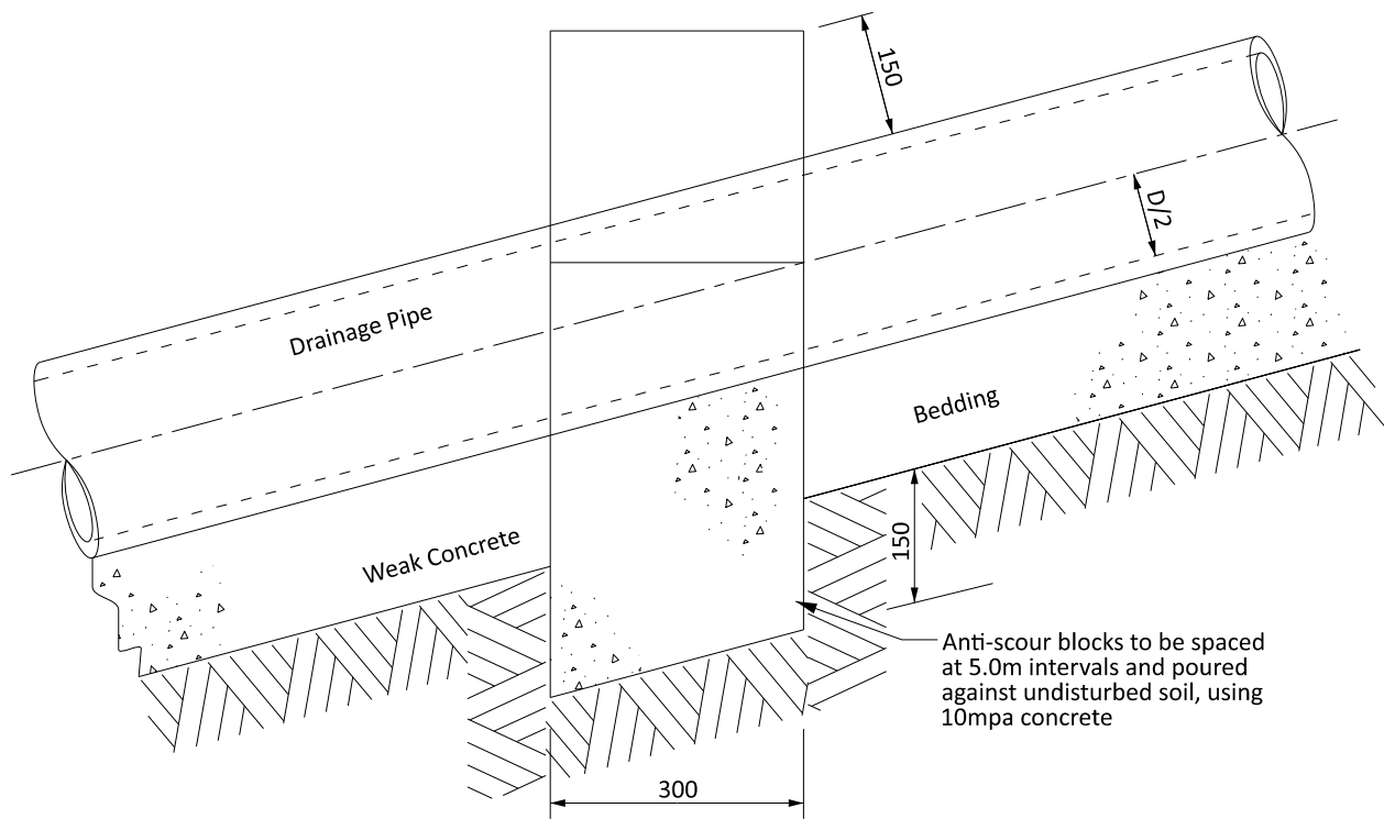
LONG SECTION
