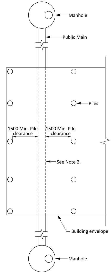
PLAN: BUILDING OVER A PUBLIC MAIN (Only permitted if an alternative alignment is not possible)
