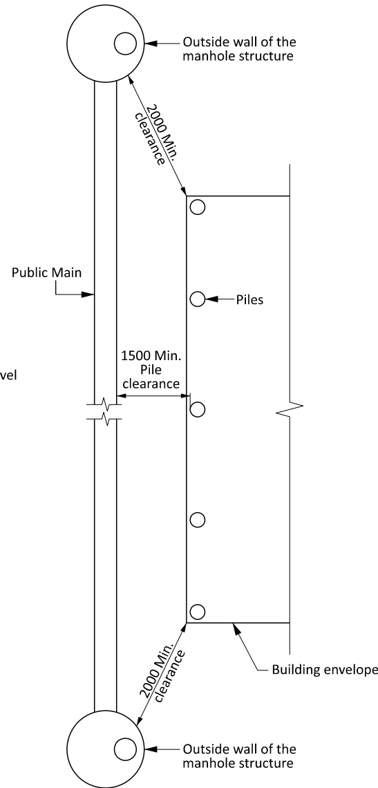
PLAN: BUILDING ADJACENT TO A PUBLIC MAIN
