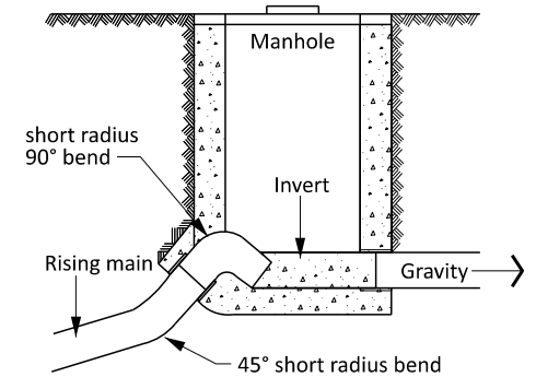
DETAIL A - ENTRY INTO RECEIVING MANHOLE
