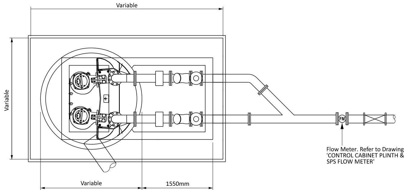
SECTIONAL PLAN
