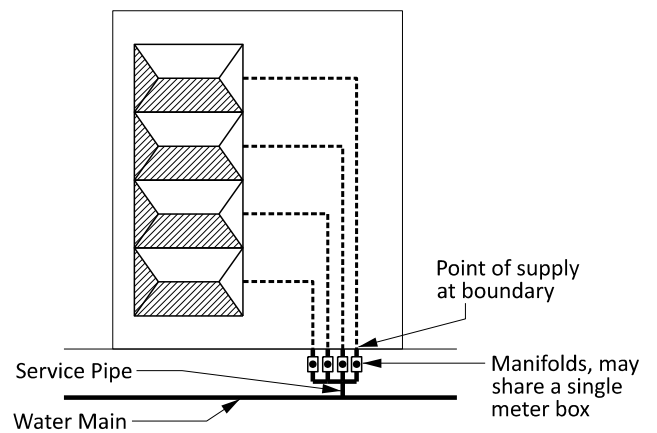
2 to 4 CUSTOMERS Single Lot - Manifold Connection
