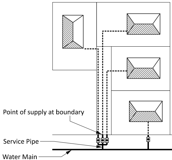
2 to 4 CUSTOMERS Right of Way - Manifold Connection
