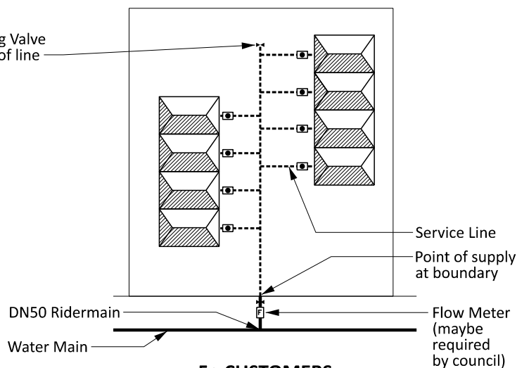
5+ CUSTOMERS Single Lot - Ridermain
