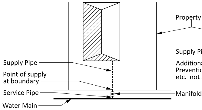
SINGLE PROPERTY Single Connection
