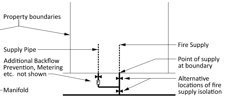
SINGLE PROPERTY Single Connection with Fire Connection
