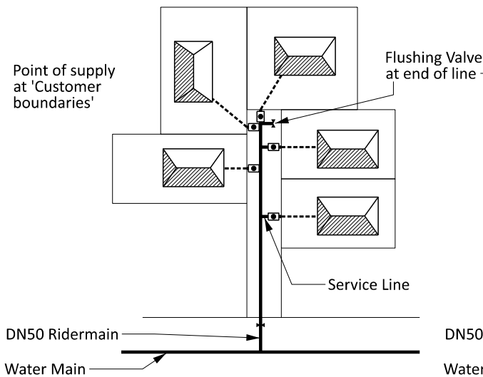
5+ CUSTOMERS Accessway - Ridermain
